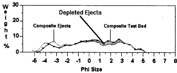
Fig. 4. Size-frequency histogram for composite test bed materials (solid curve with circles at data points) and for composite ejecta/sweep-up samples (dashed curve). The hatched area shows the size range where the composite ejecta are depleted compared to the composite test-bed. The phi ( \phi ) size scale is logarithmic ( \phi = -\log_2(\text{diameter in millimeters}) ) such that 0\phi = 1 mm, -4\phi = 16 mm, and 4\phi = 0.063 mm.
